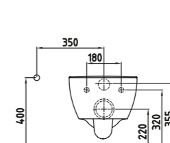
FORTE WALLHUNG WC PAN 52 cm NO-RIM CONCEALED FIXING HRKA052N3VPOW3QA0 530x350 mm
